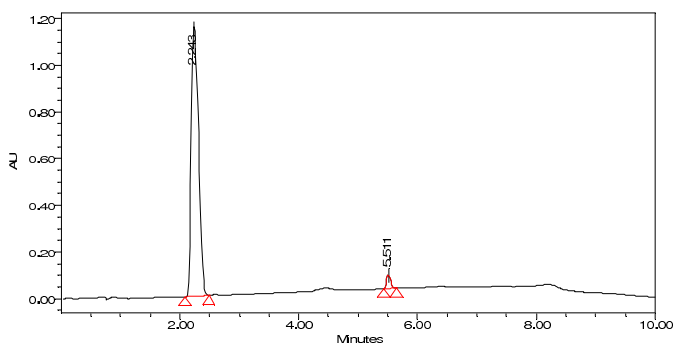
UV chromatogram
