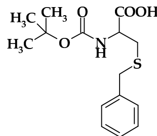
S-benzyl Boc-L-Cysteine
