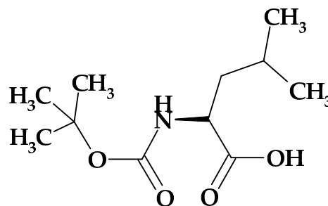
Boc-L-Leucine
