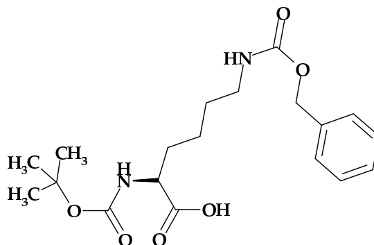
Boc-L-Lysine(Z)
