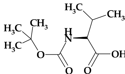
Boc-L-Valine
