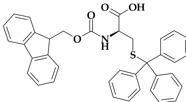
S-Trityl Fmoc-D-Cysteine
