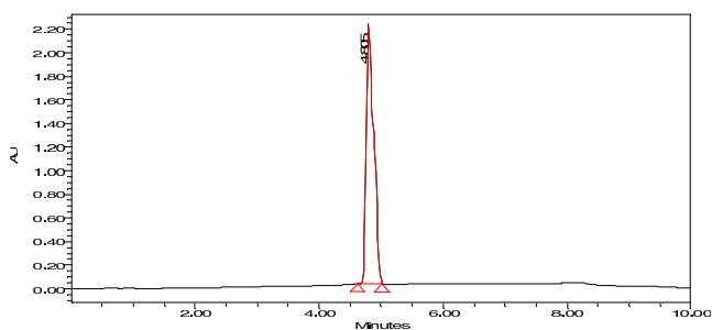
UV chromaotgram
