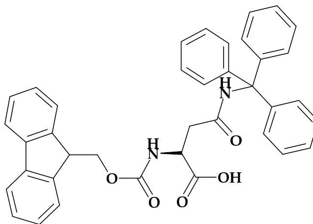
Fmoc-L-Asparagine(Trt)
