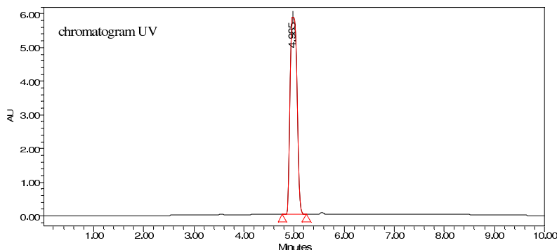
Fmoc-L-Glutamic acid \gamma - tert-Butyl ester
