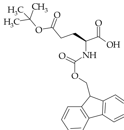
Fmoc-L-Glutamic acid \gamma - tert-Butyl ester
