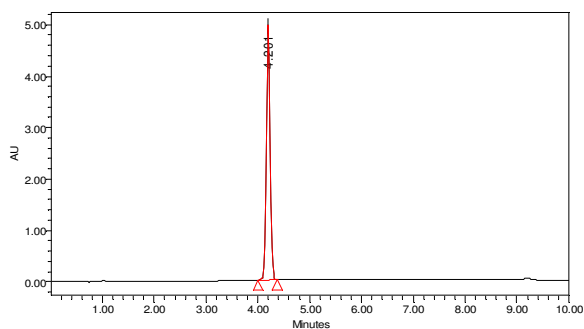
UV chromatogram
