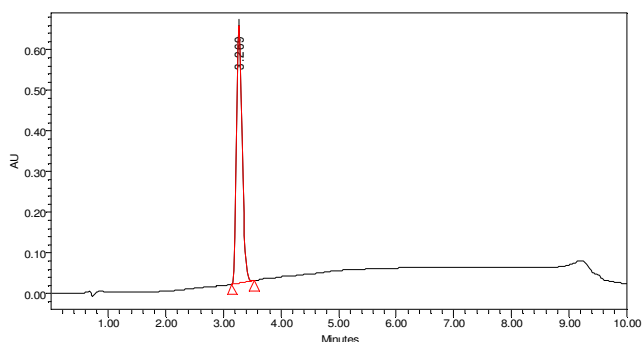
UV chromatogram
