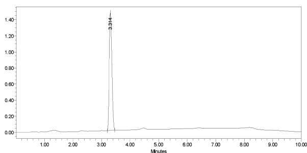
UV chromatogram
