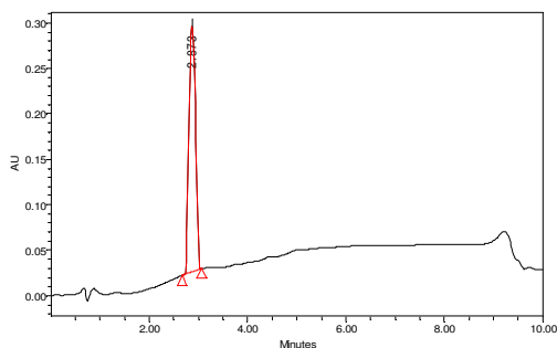
UV chromatogram
