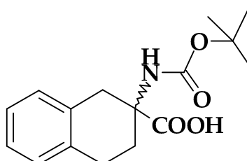
N-BOC-DL-2-Aminotetralin-2-carboxylic acid
