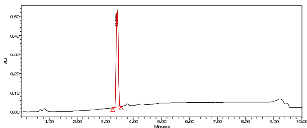
UV chromatogram
