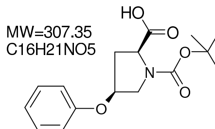
(2S,4S)-Boc-4-phenoxy-pyrrolidine-2-carboxylic acid
