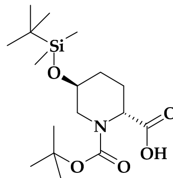
(+/-)-trans-Boc-5-hydroxypipelic acid t-butyl dimethylsilyl ether
