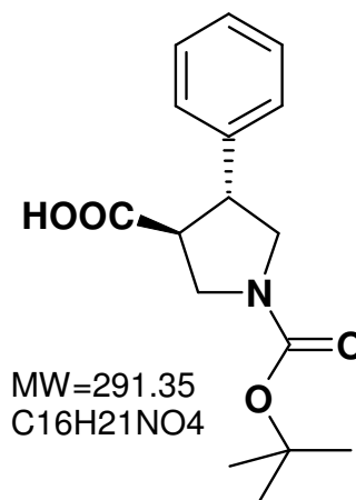
trans-3-Carboxy-4-phenyl-1-Boc-pyrrolidine
