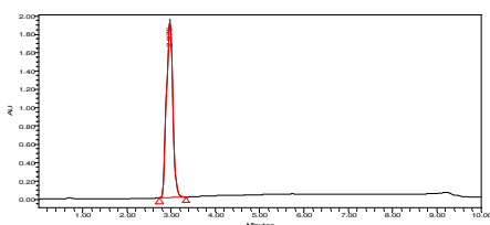
UV chromatogram
