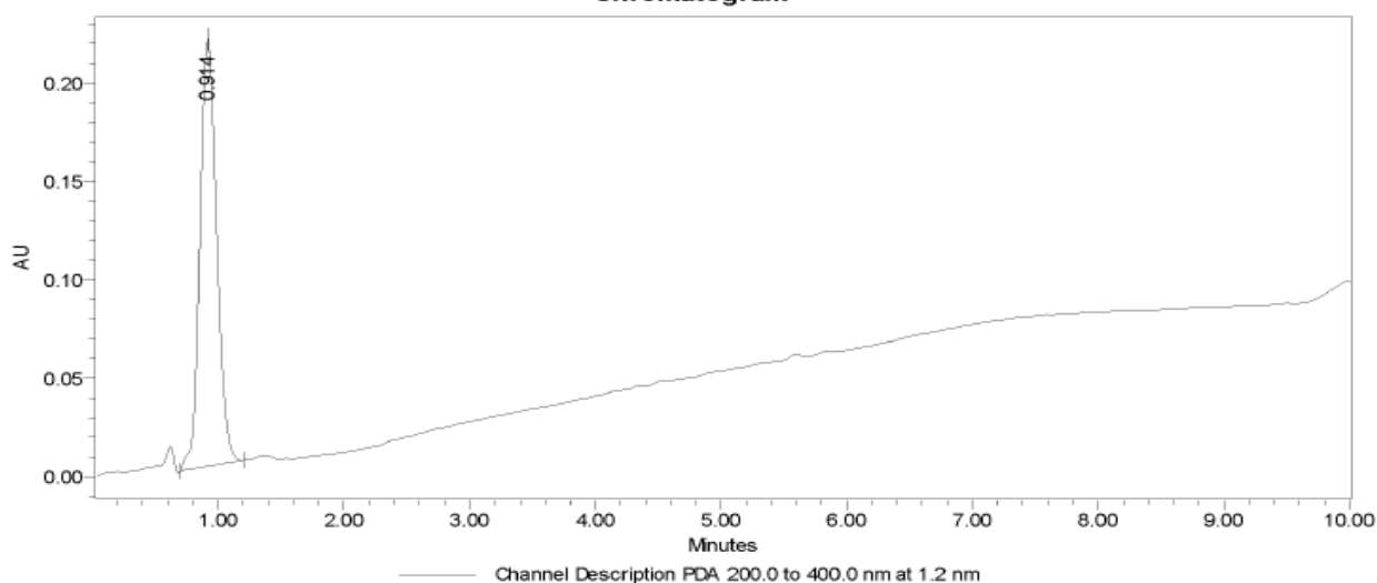
Chromatogram
