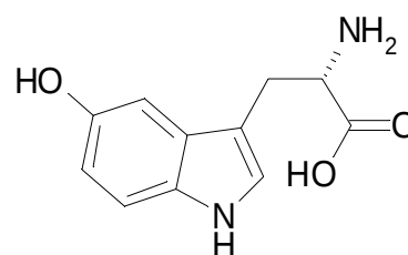
L-5-hydroxy-tryptophan
